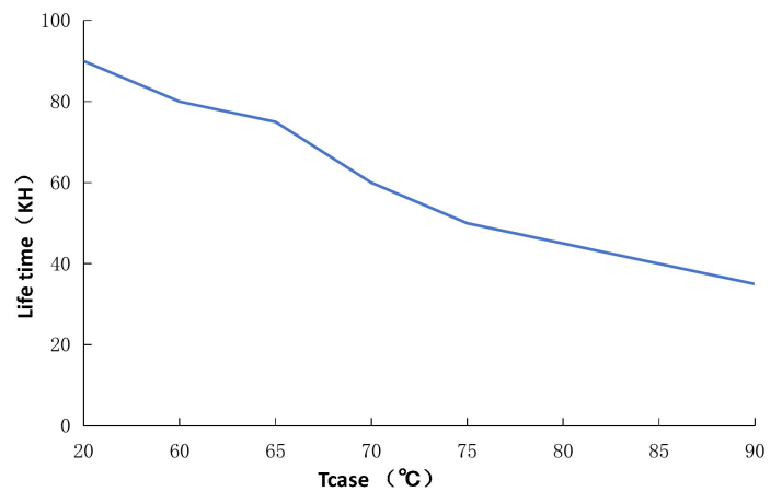
Tcse VS Life time
