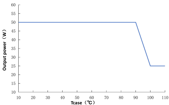
Output power VS Tcse
