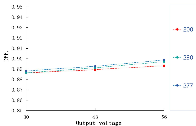
Eff. VS Output voltage
