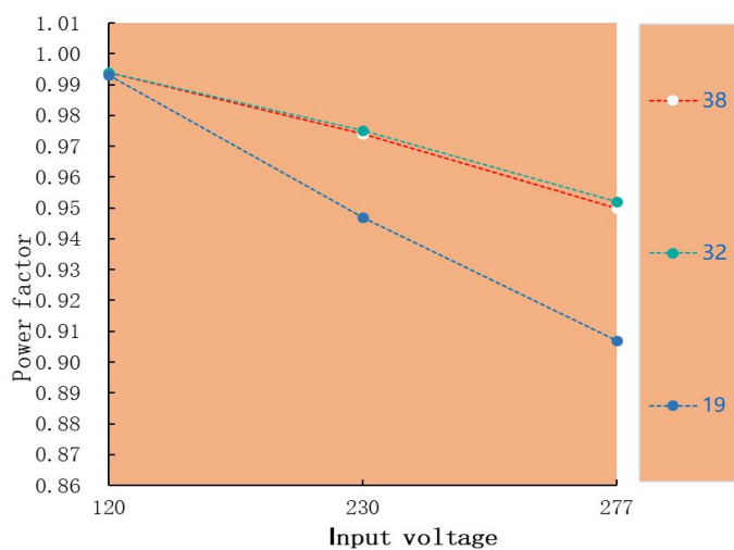
Power factor VS Input voltage HAE-150W-38A( II )
