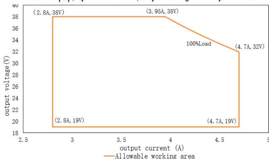
HAE-150W-38A(II)(Import:120-277Vac)output voltage VS output current
