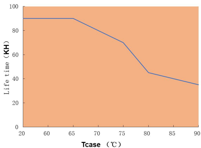
Tcase VS Life time HAE-150W-38/56A( II )
