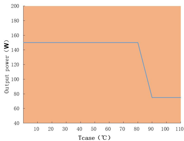
Output power VS Tcase HAE-150W-38/56A( II )
