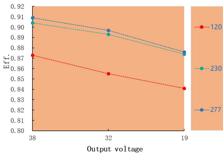
Eff. VS Output voltage HAE-150W-38A(II)
