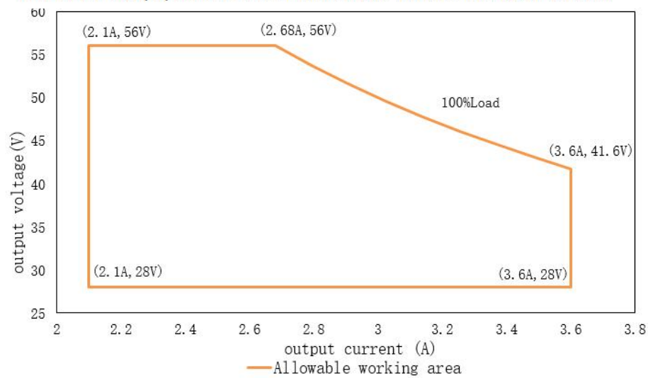
HAE-150W-56A(II)(Import:120-277Vac)output voltage VS output current
