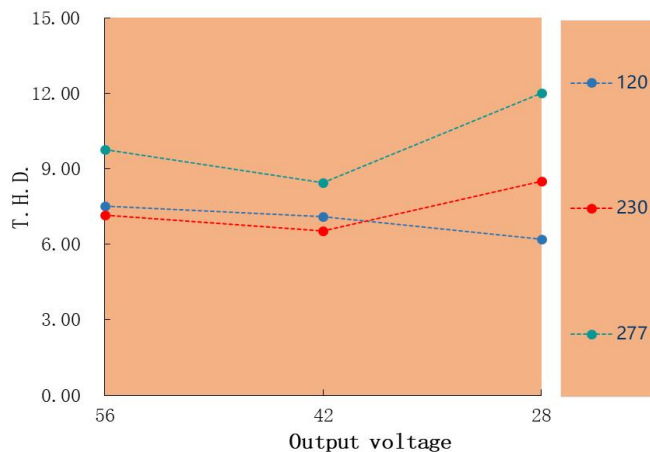
T.H.D. VS Output voltage HAE-150W-56A( II )
