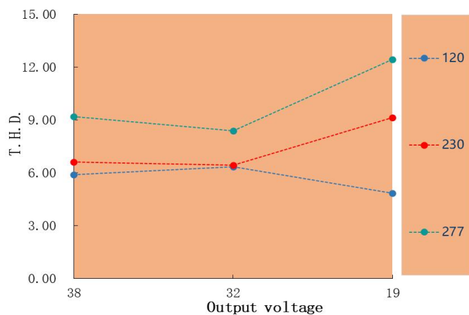
T.H.D. VS Output voltage HAE-150W-38A( II )
