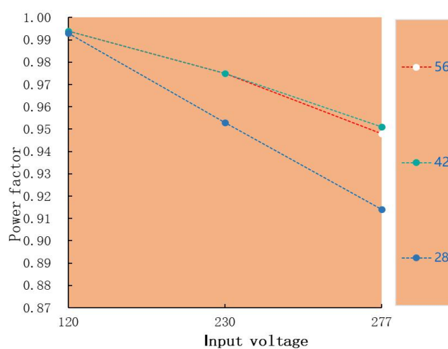
Power factor VS Input voltage HAE-150W-56A( II )
