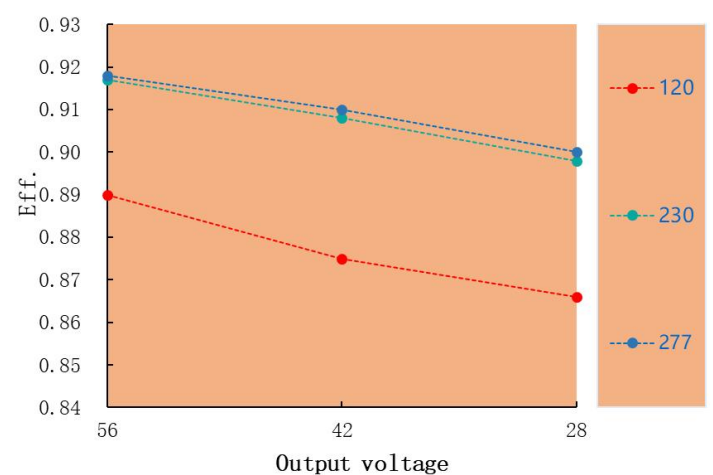
Eff. VS Output voltage HAE-150W-56A(II)
