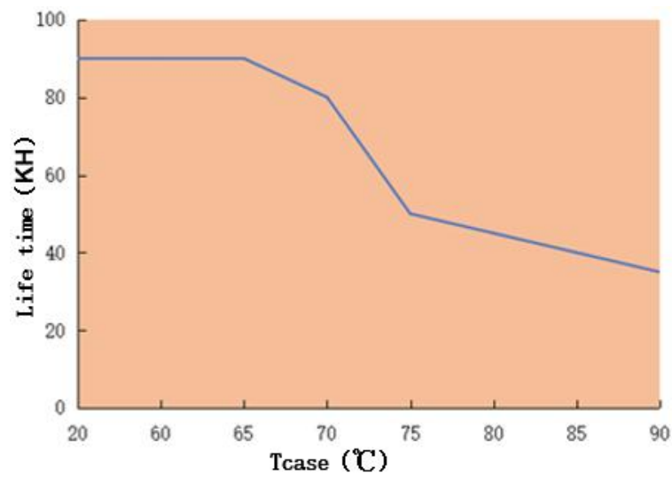
Tcase VS Life time LAG-150H-470A
