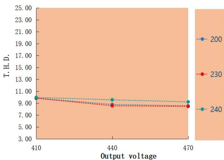
T.H.D. VS Output voltage LAG-150H-470A
