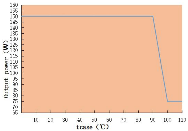
Output power VS Tcase LAG-150H-470A
