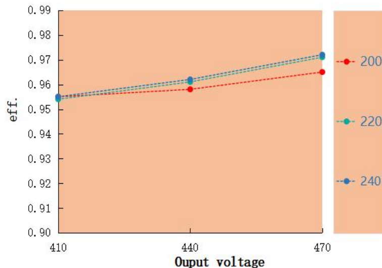
Eff. VS Output voltage LAG-150H-470A-XP
