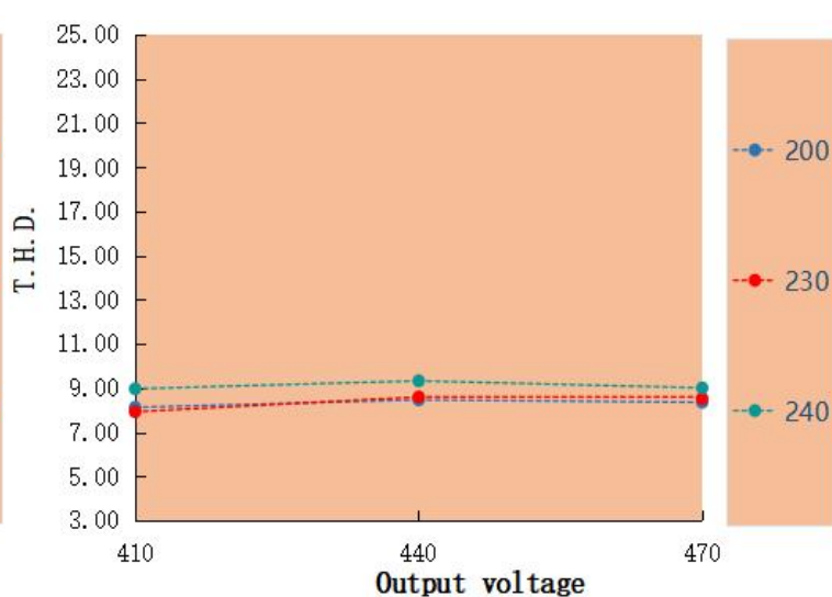
T.H.D. VS Output voltage LAG-150H-470A-XP
