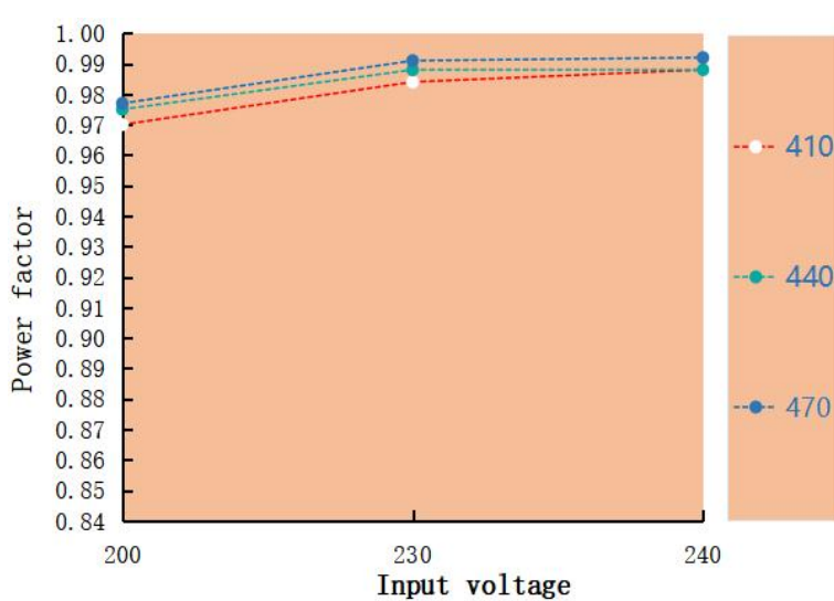
Power factor VS Input voltage LAG-100H-470A-XP
