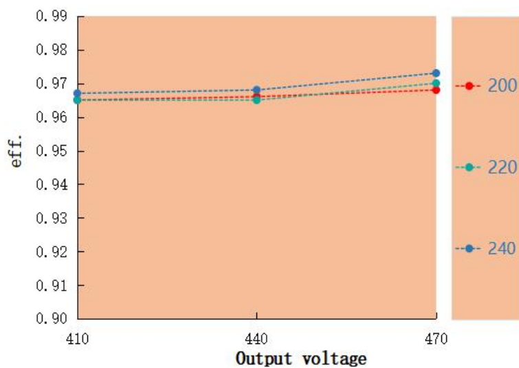
Eff. VS Output voltage LAG-100H-470A-XP
