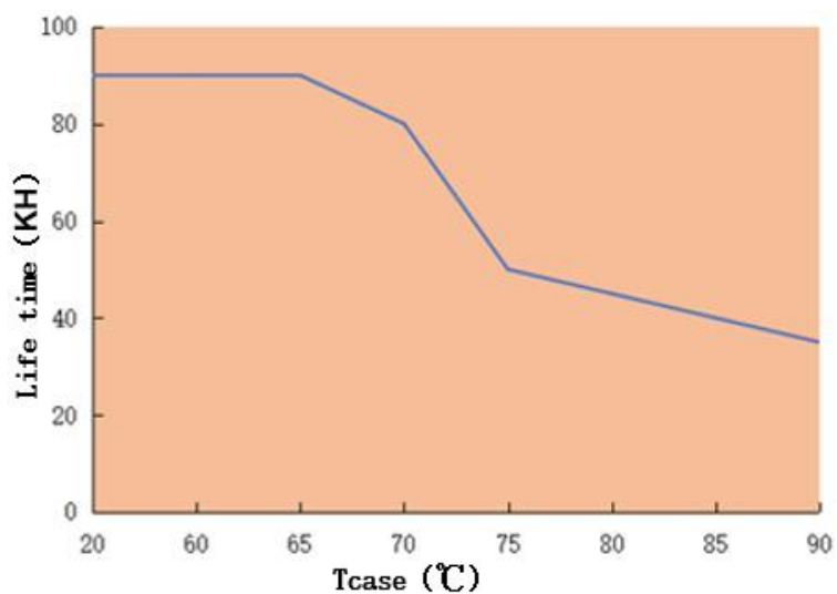
Tcase VS Life time LAG-100H-470A
