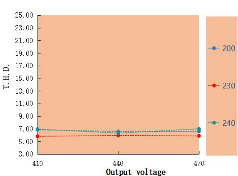
T.H.D. VS Output voltage LAG-100H-470A
