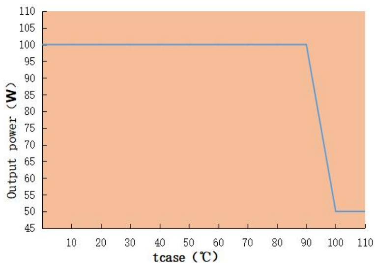
Output power VS Tcase LAG-100H-470A
