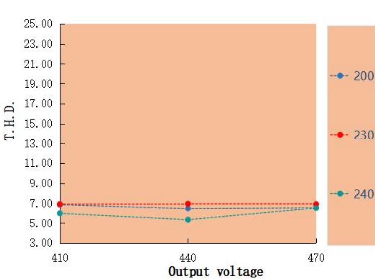
T.H.D. VS Output voltage LAG-100H-470A-XP
