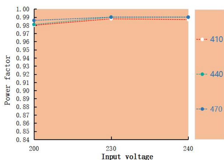
Power factor VS Input voltage LAG-100H-470A
