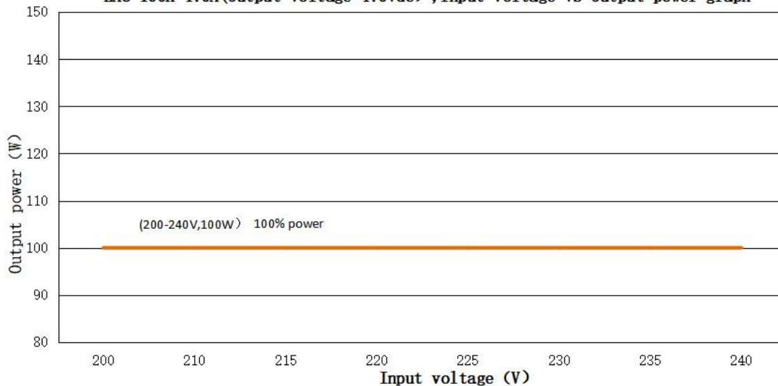
LAG-100H-470A(Output voltage=470Vdc) , Input voltage VS Output power graph
