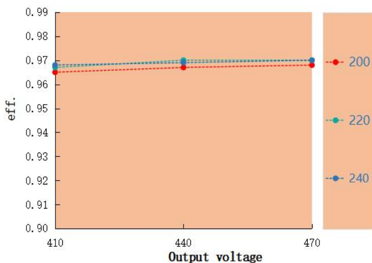
Eff. VS Output voltage LAG-100H-470A
