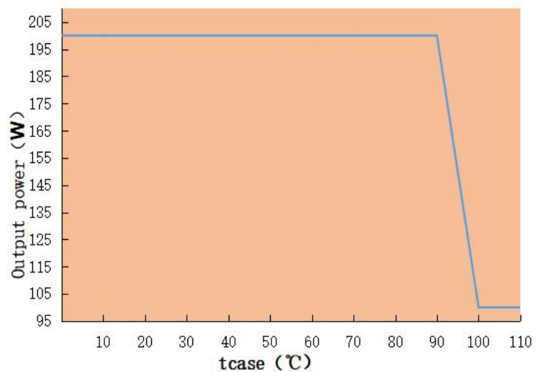
Output power VS Tcase LAG-200H-470A
