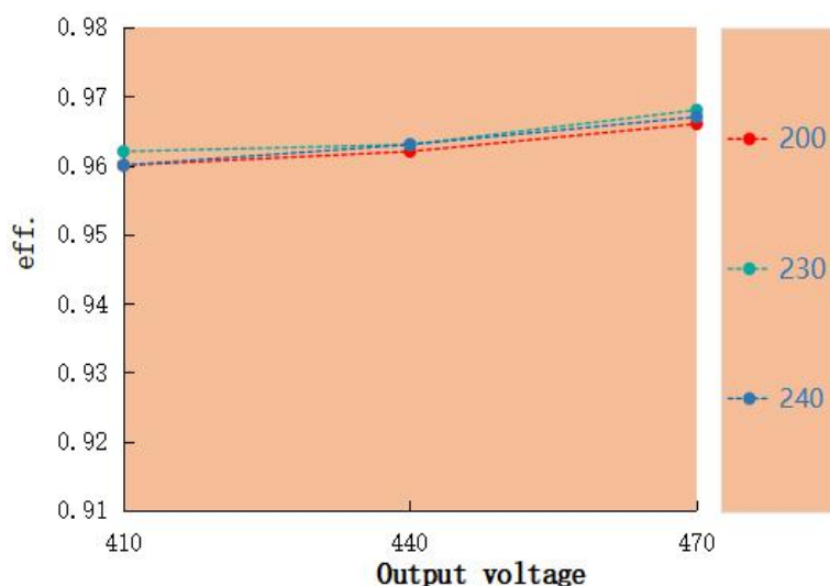
Eff. VS Output voltage LAG-200H-470A
