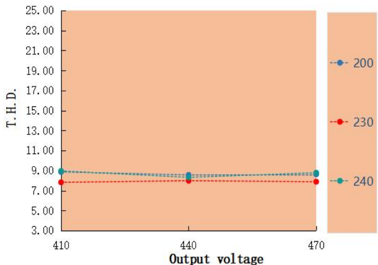
T.H.D. VS Output voltage LAG-200H-470A
