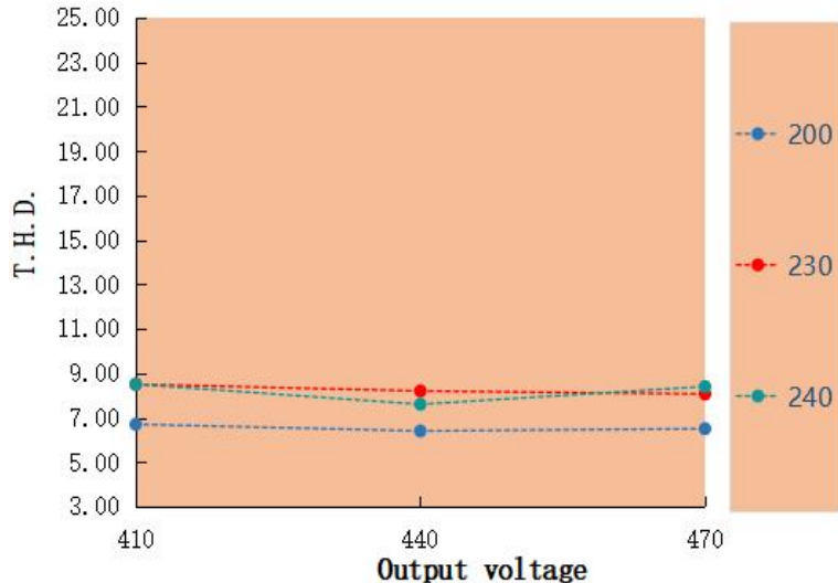
T.H.D. VS Output voltage LAG-200H-470A-XP
