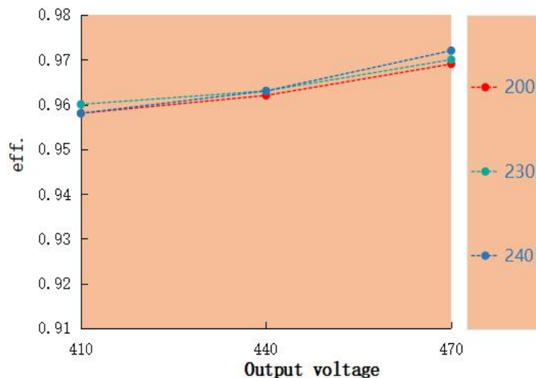
Eff. VS Output voltage LAG-200H-470A-XP
