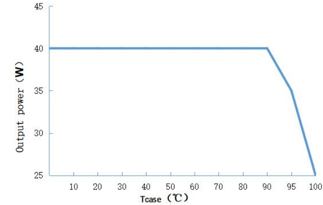
Output power vs. ambient temperature curve
