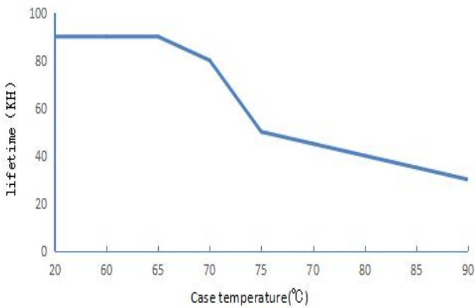
Tc VS Life (HAE-40W)
