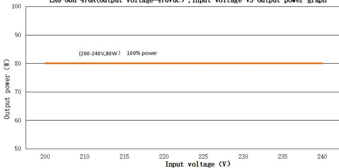
LAG-80H-470A(Output voltage=470Vdc) , Input voltage VS Output power graph
