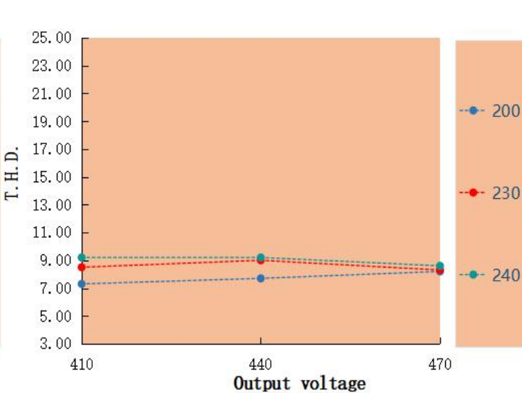
T.H.D. VS Output voltage LAG-80H-470A-XP
