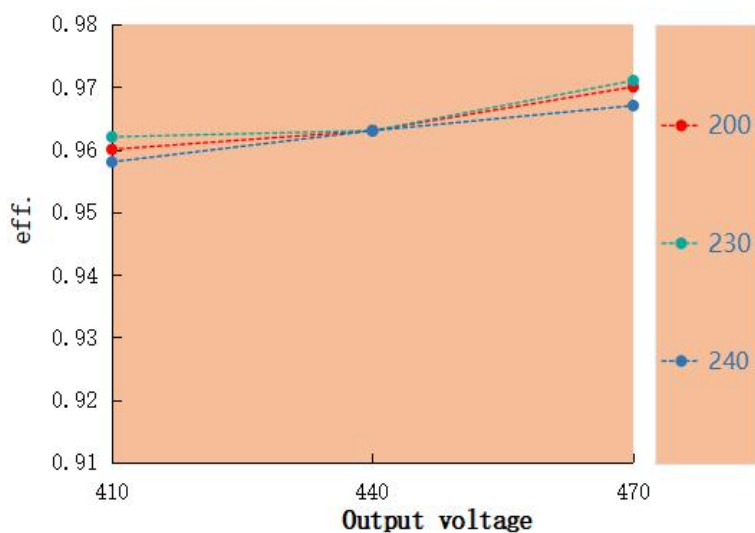
Eff. VS Output voltage LAG-80H-470A
