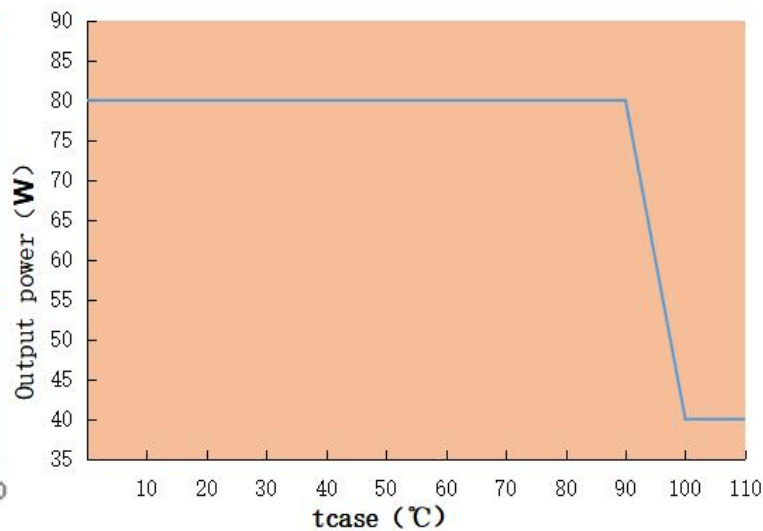
Output power VS Tcase LAG-80H-470A
