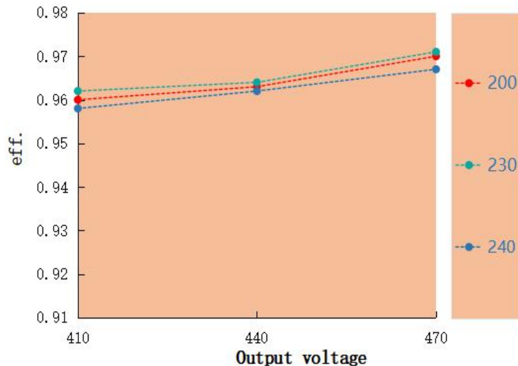
Eff. VS Output voltage LAG-80H-470A-XP
