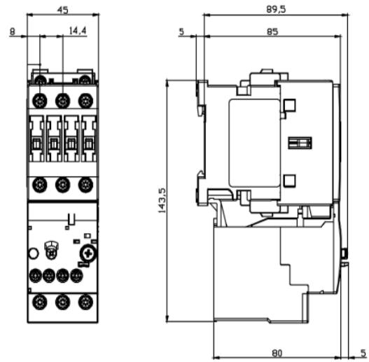
3RU7126 Mounting with contactor
