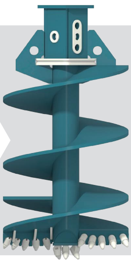
双头单螺直螺 Double head single flight straight auger
