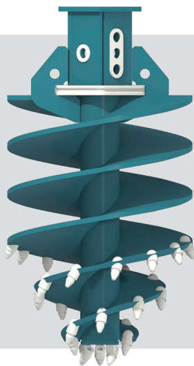
双头双螺锥螺 Double start double flight conical auger
