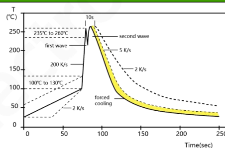
Wave soldering curve
