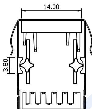
俯视图 Bottom side view
