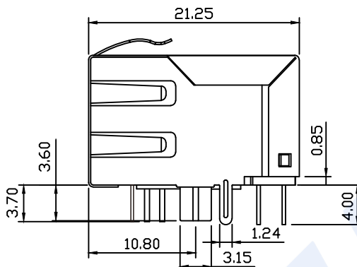
左侧视图 Left side view
