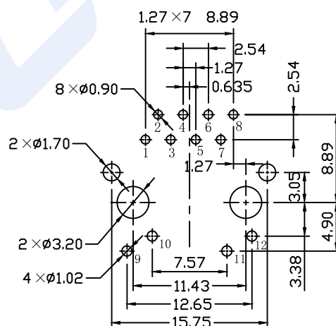
PCB布局建议(俯视图) Suggested PC Board Layout(TOP View)
