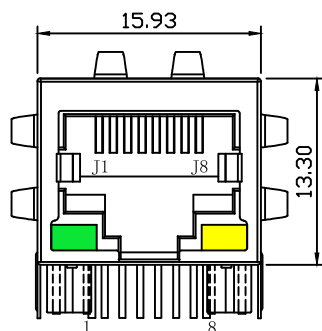
正侧视图 Front side view
