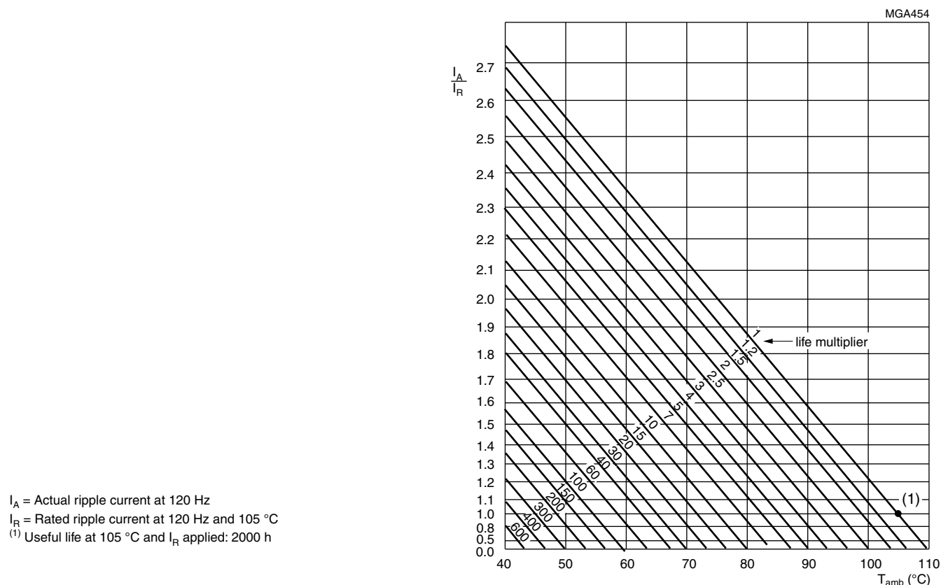
Fig. 4 - Multiplier of useful life as a function of ambient temperature and ripple current load
