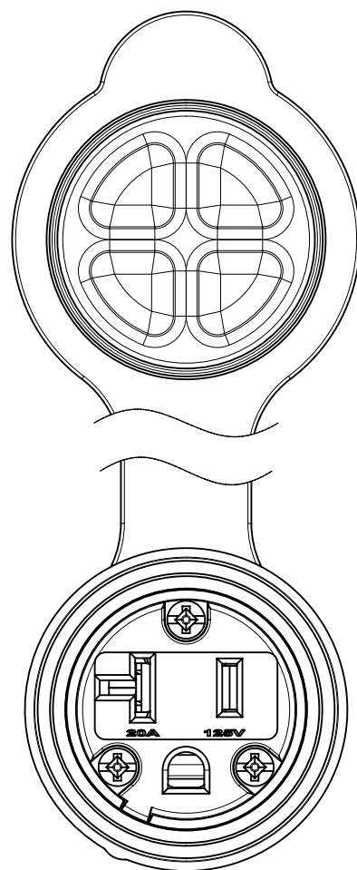
NEMA 5-20R SECONDARY WOODHEAD #15W33 CONNECTOR
