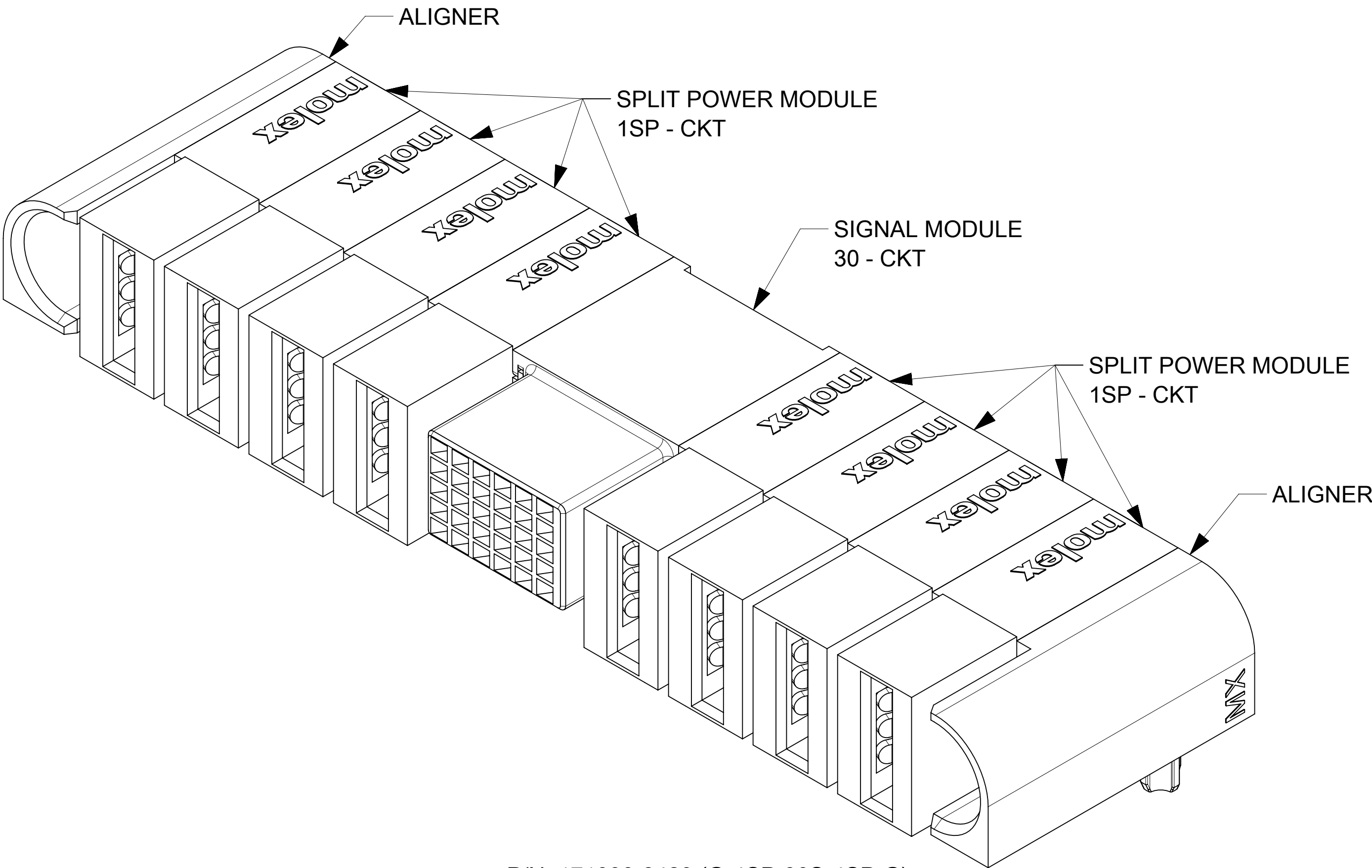
P/N: 171090-8429 (G-4SP-30S-4SP-G)
