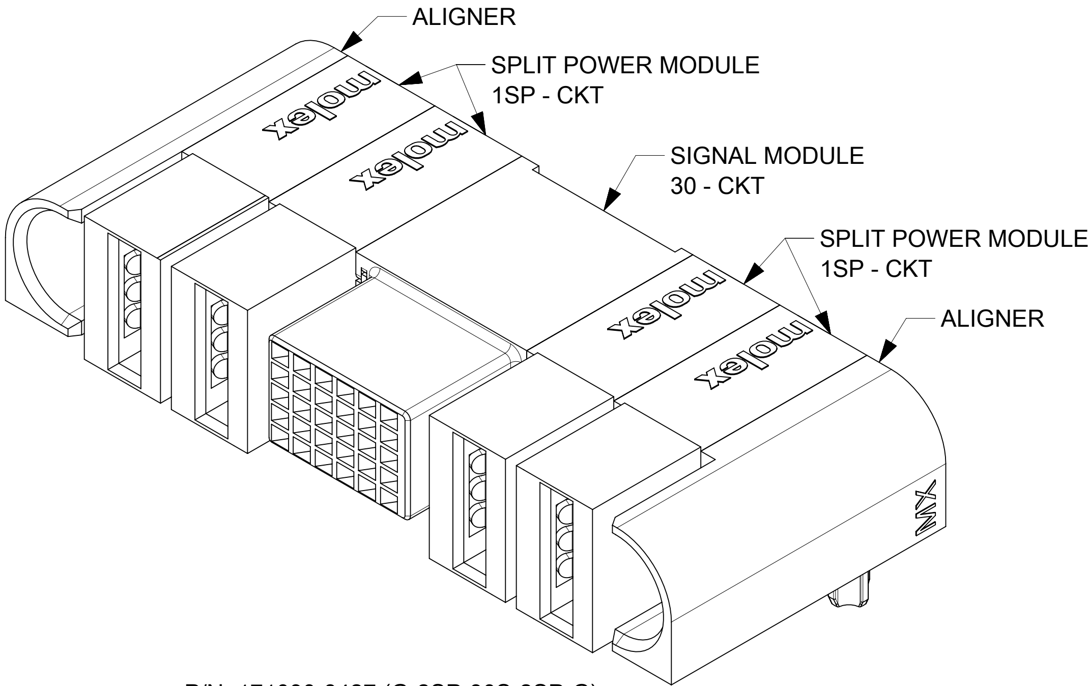
P/N: 171090-8427 (G-2SP-30S-2SP-G)
