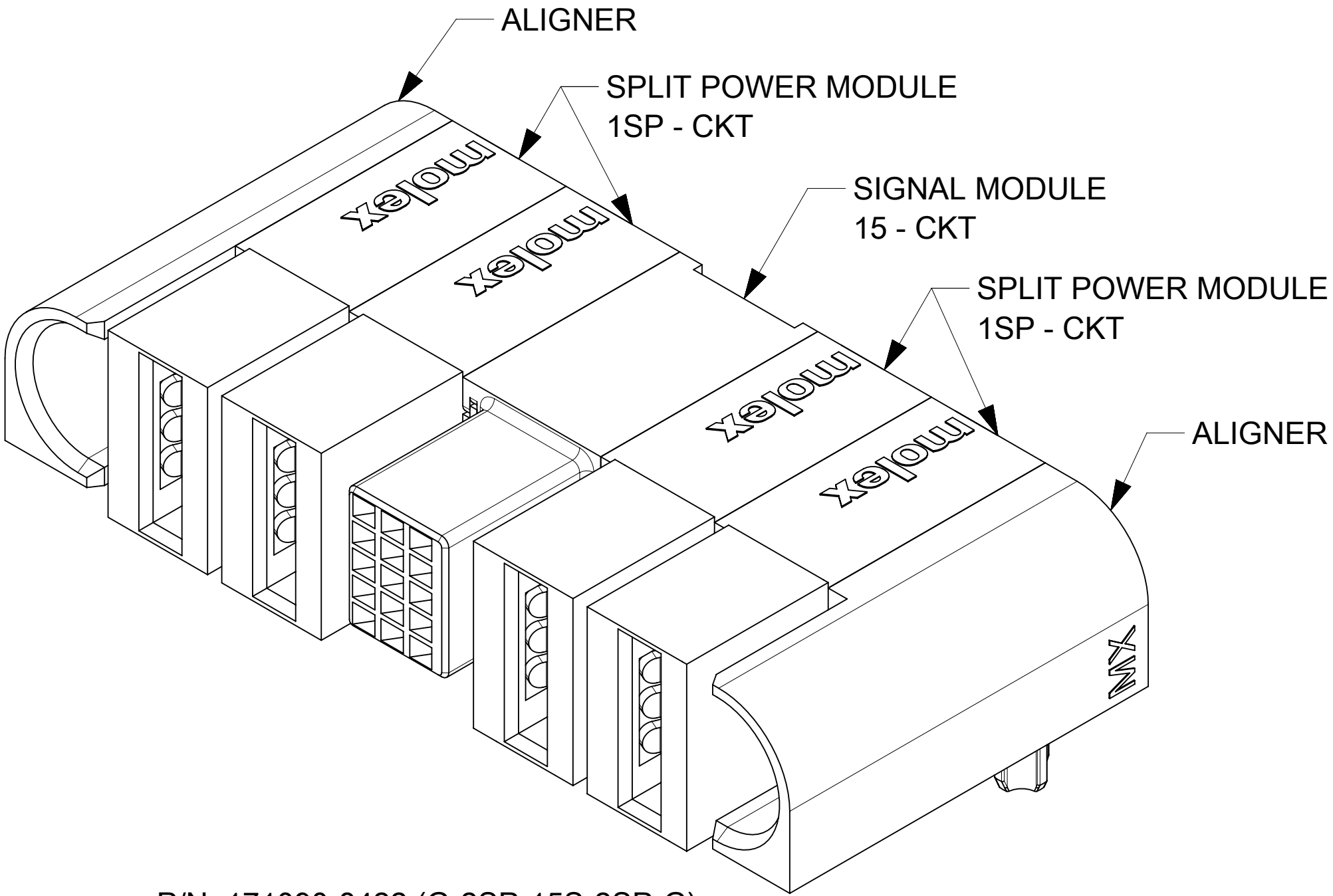
P/N: 171090-8422 (G-2SP-15S-2SP-G)
