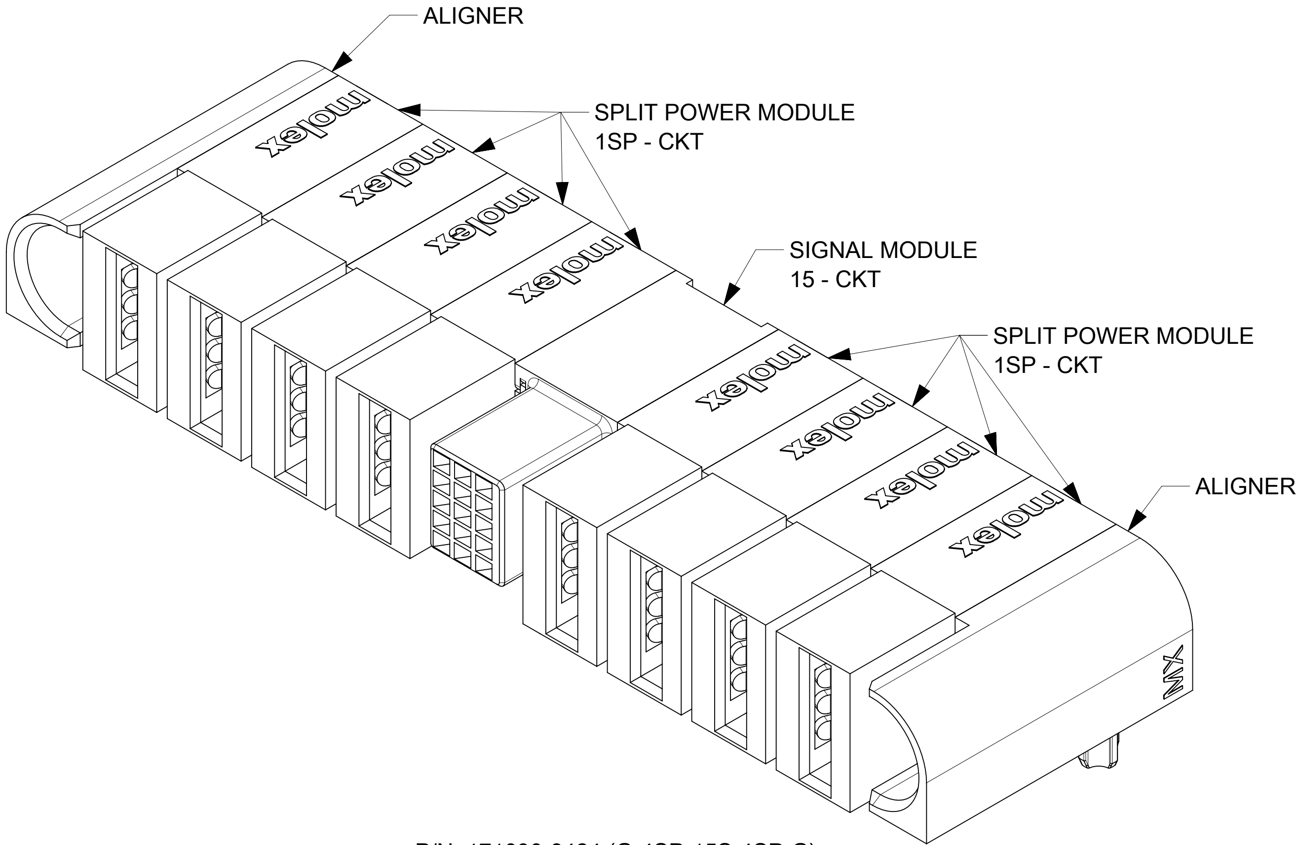
P/N: 171090-8424 (G-4SP-15S-4SP-G)
