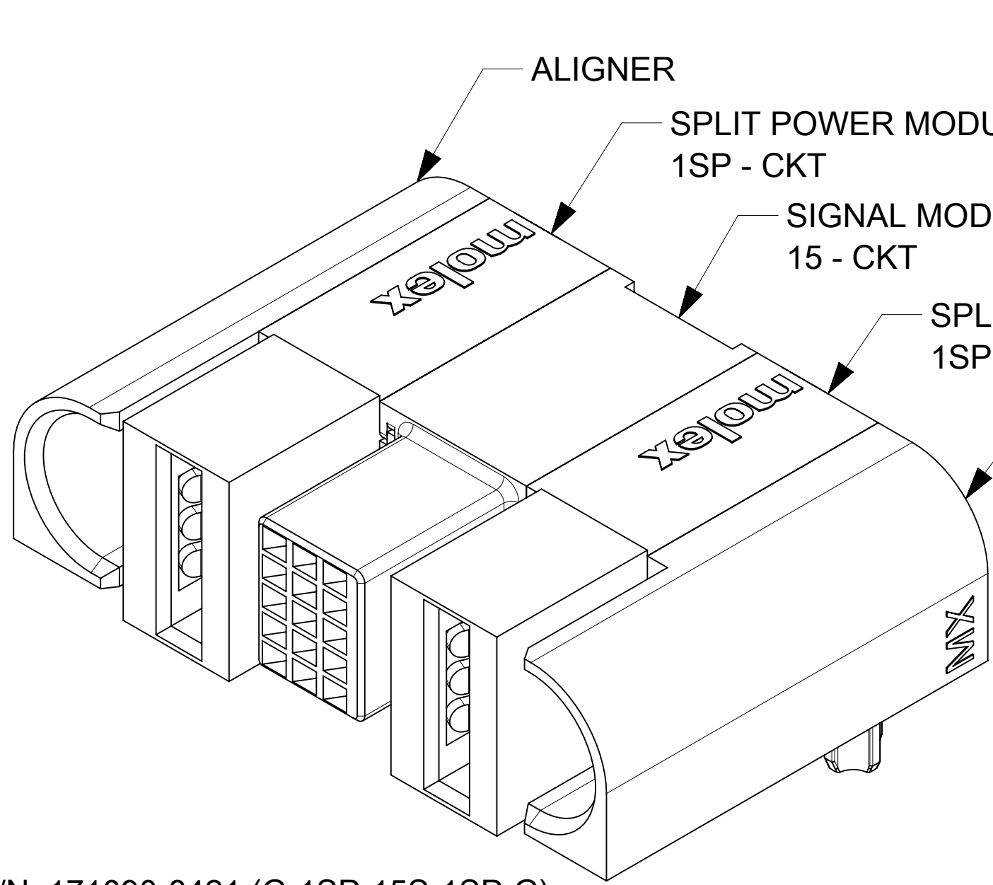
P/N: 171090-8421 (G-1SP-15S-1SP-G)
