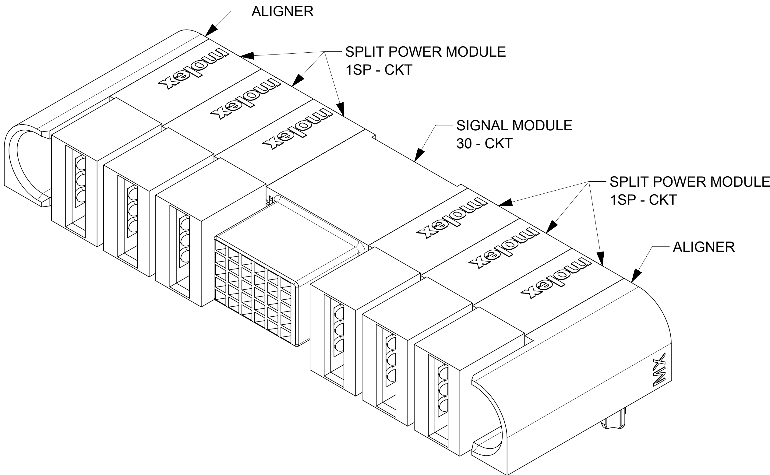
P/N: 171090-8428 (G-3SP-30S-3SP-G)
