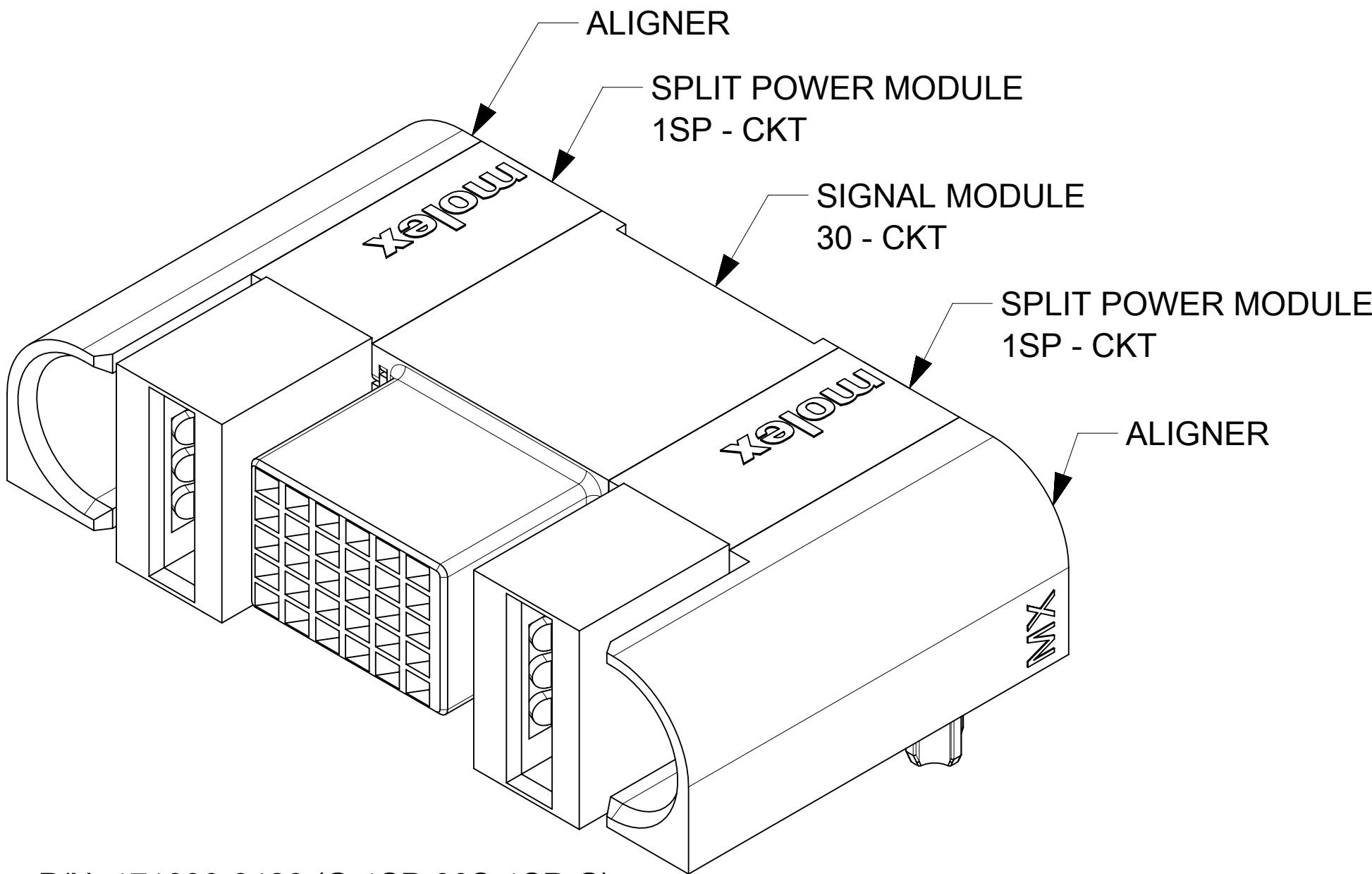
P/N: 171090-8426 (G-1SP-30S-1SP-G)
