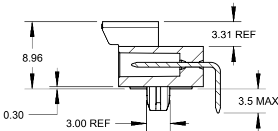
SECTION Y-Y
