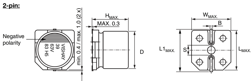
Fig. 2 - Dimensional outline
