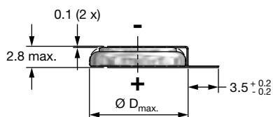
Fig. 6 - Form D2: Surface Mount Flat (single cell, keyed polarity)
