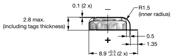
Fig. 5 - Form D1: Surface Mount Flat (single cell, keyed polarity)
