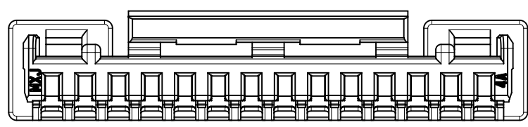
VIEW Y 14-16極 14-16 CIRCUIT
