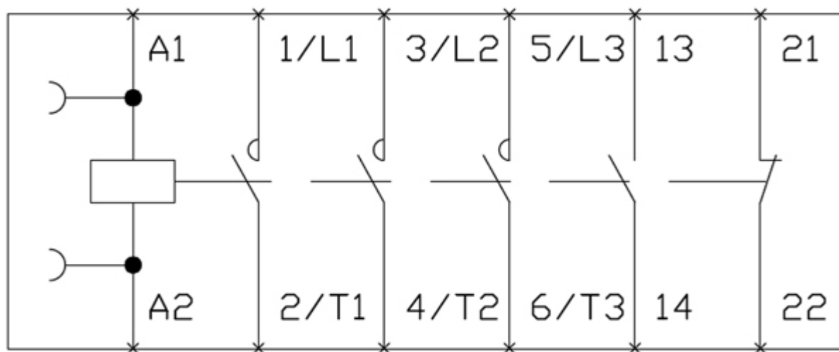
LEN00C003 Wiring Diagram
