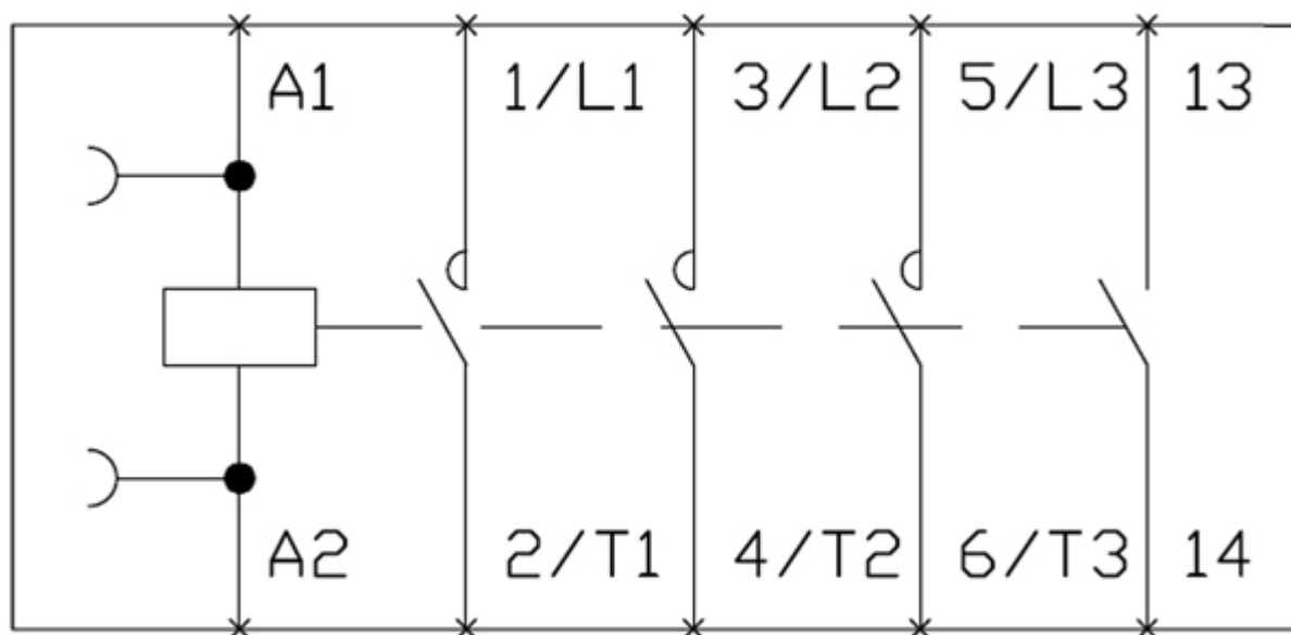
LENO02B003 Wiring Diagram
