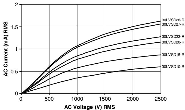
AC CURRENT VS. VOLTAGE (Typical)
