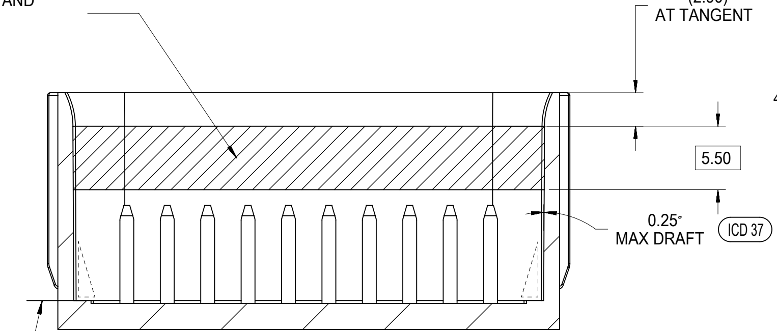
SECTION B-B
