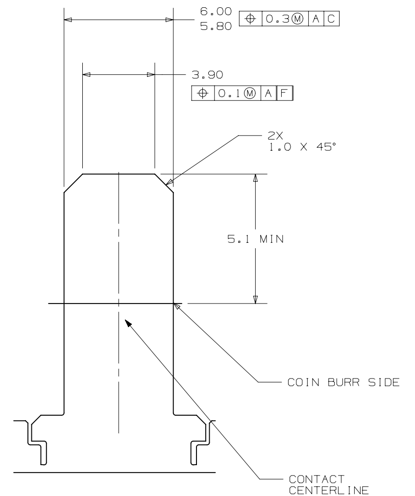
SECTION CB-CB
