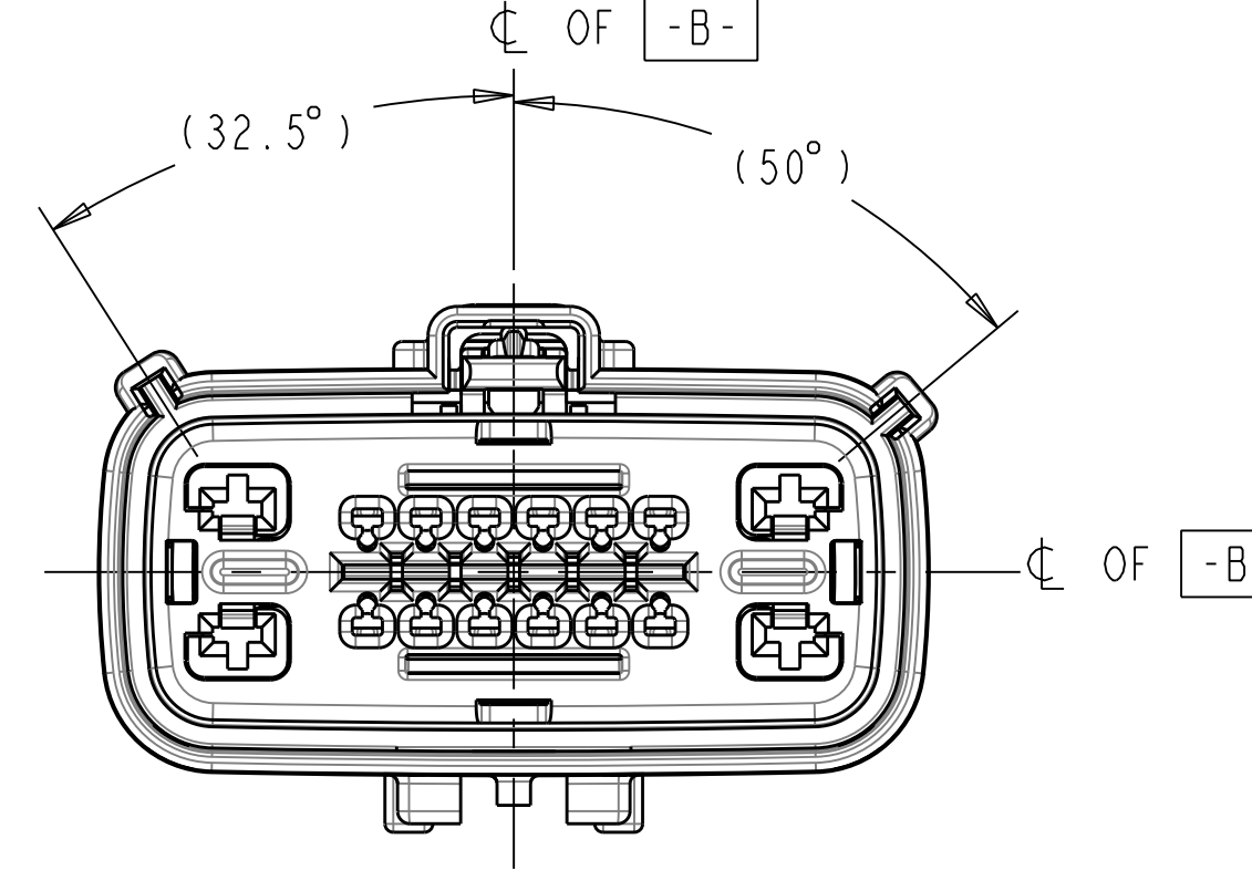
KEYING OPTION H SCALE 2:1
