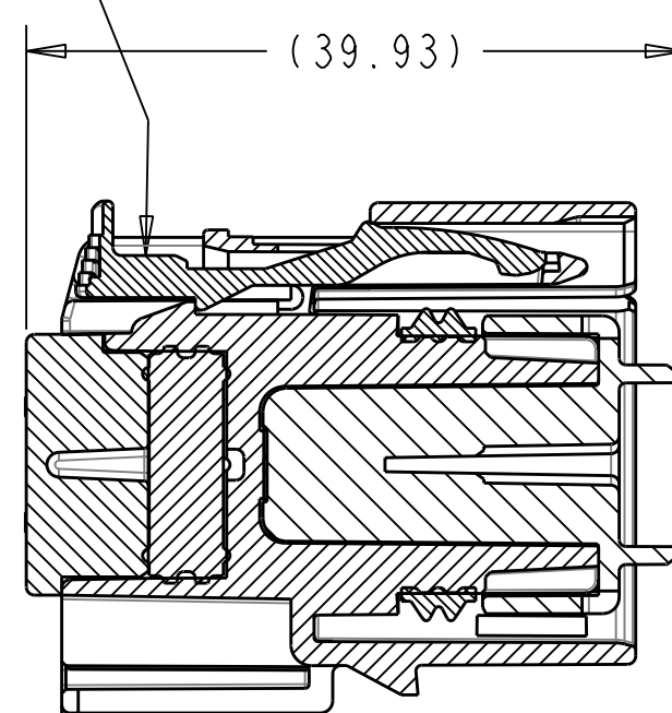
SECTION B-B (RECEPTACLE INSERT WITH SHORTING BAR LIFTER SHOWN IN FULL-LOCK) SEE NOTE #2
