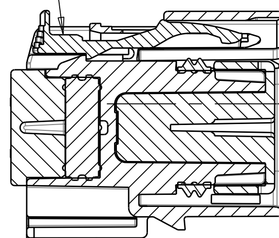
SECTION B-B (RECEPTACLE INSERT SHOWN IN FULL-LOCK) SEE NOTE #2
