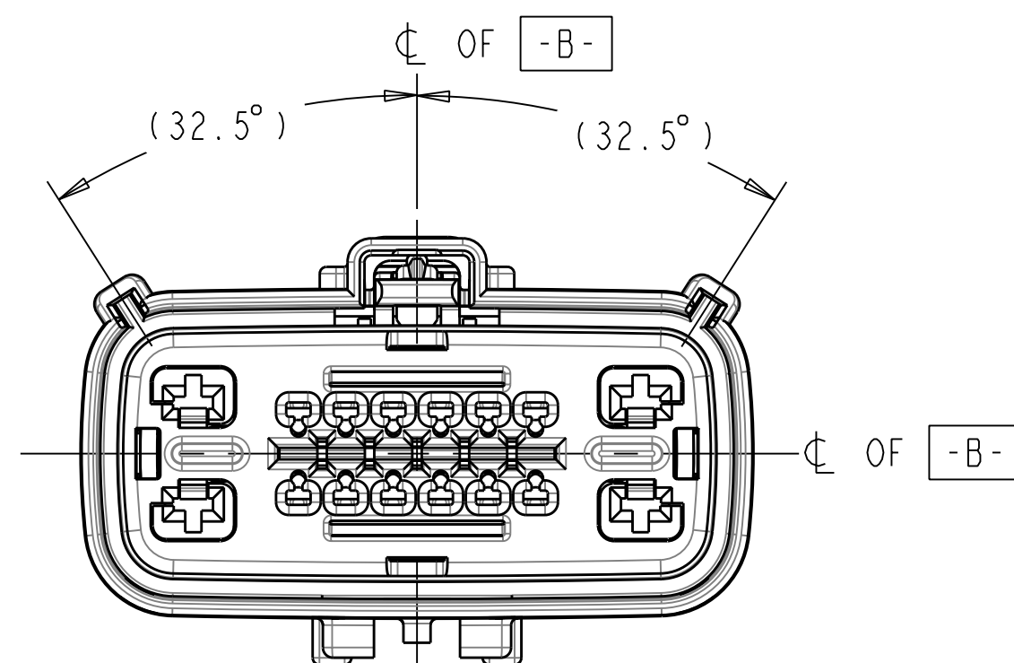
KEYING OPTION E SCALE 2:1
