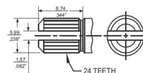
K – Split Knurl
