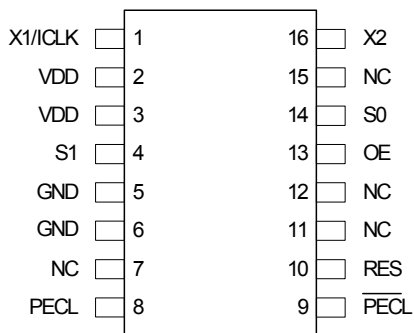
16 Pin (150 mil) SOIC
