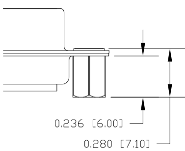
2 ..... 0.236" SOLDER SIDE
