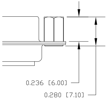
3 ..... 0.236" MATING SIDE
