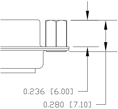
3 ..... 0.236" MATING SIDE
