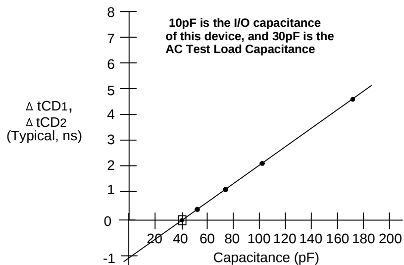
Figure 3. Typical Output Derating (Lumped Capacitive Load).
