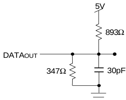
Figure 1. AC Output Test load.
