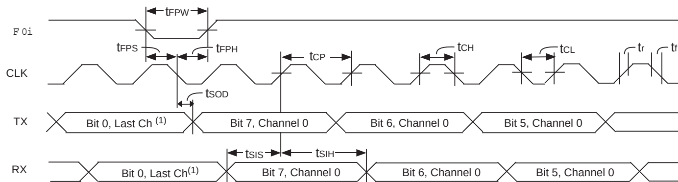
Figure 7. ST-BUS® Timing
