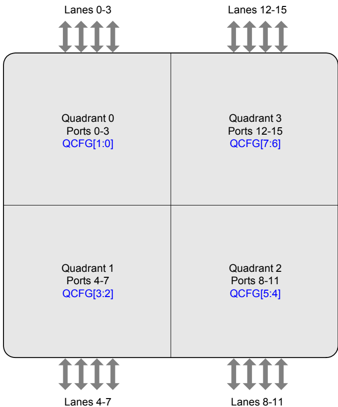
Figure 2: Quadrant Configuration using QCFG[7:0]
