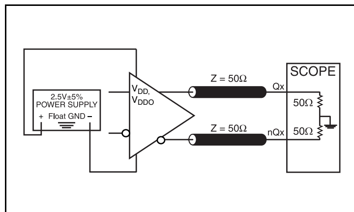
2.5V Core/2.5V LVDS Output Load Test Circuit
