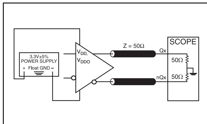
3.3V Core/3.3V LVDS Output Load Test Circuit
