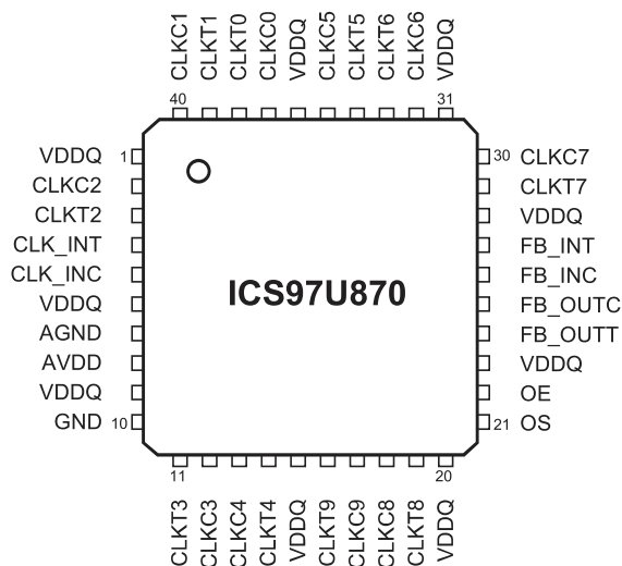
40-Pin MLF
