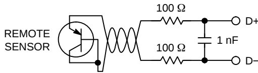
Figure 35. Filter Between Remote Sensor and ADT7462
