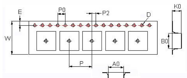
Tape Dimensions
