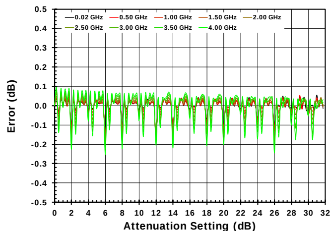
Figure 19. Step Accuracy vs Attenuator Setting [LSB = 0.50dB]
