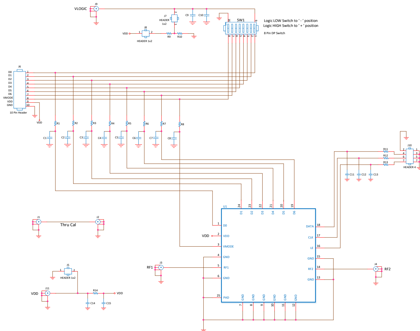
Figure 37. Electrical Schematic
