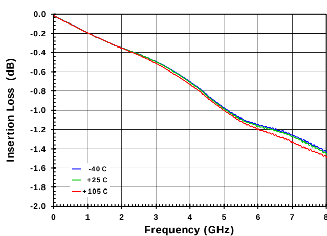
Figure 27. Evaluation Board Insertion Loss
