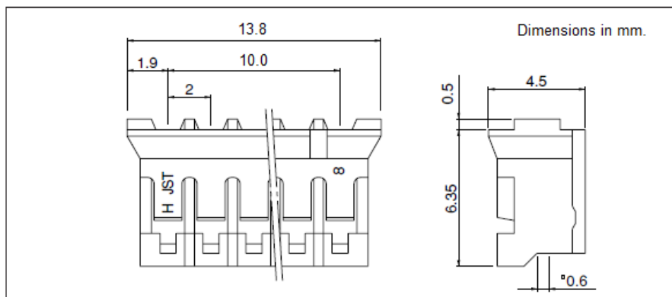
Figure 2. Receptacle Drawing
