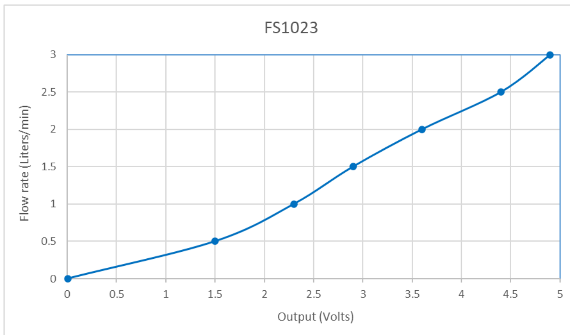
Figure 1. Analog Output Curve (in Water, Room Temperature)
