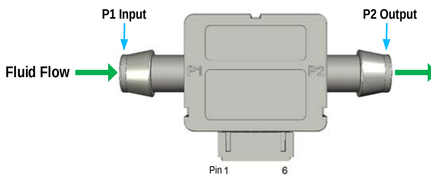
FS1025 Pin Assignments – Top View
