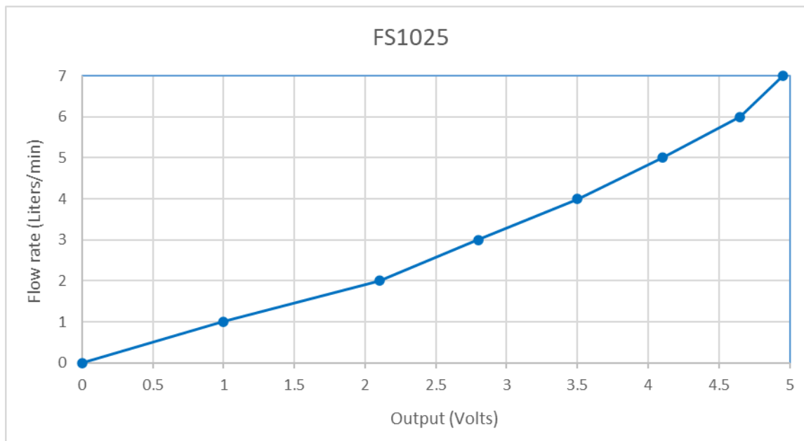
Figure 1. Analog Output Curve (in Water, Room Temperature)
