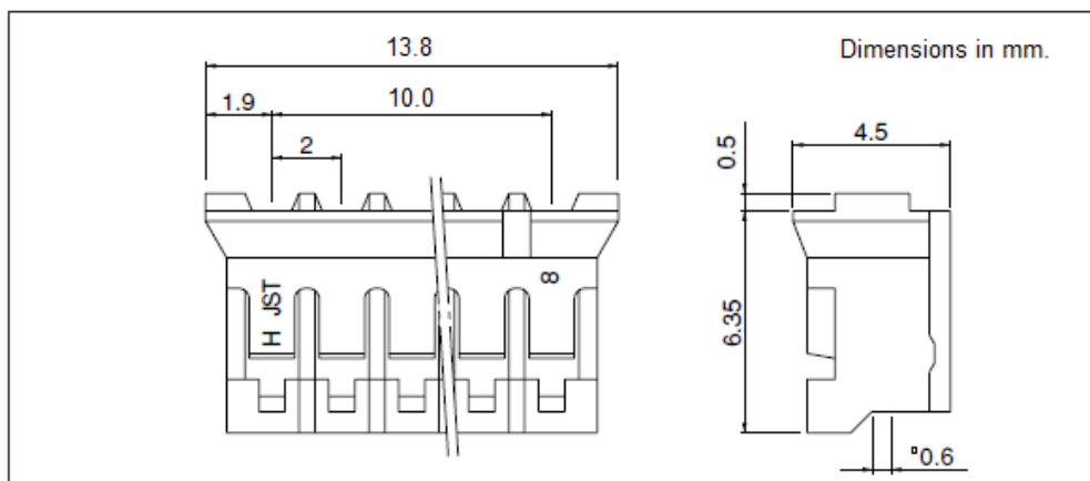
Figure 2. Receptacle Drawing
