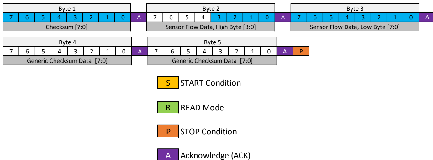
Figure 6. Flow Data from FS1027-DG
