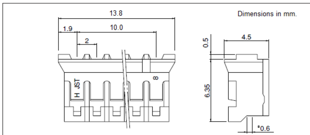
Figure 2. Receptacle Drawing
