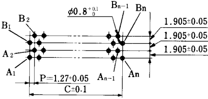
Mating Side
