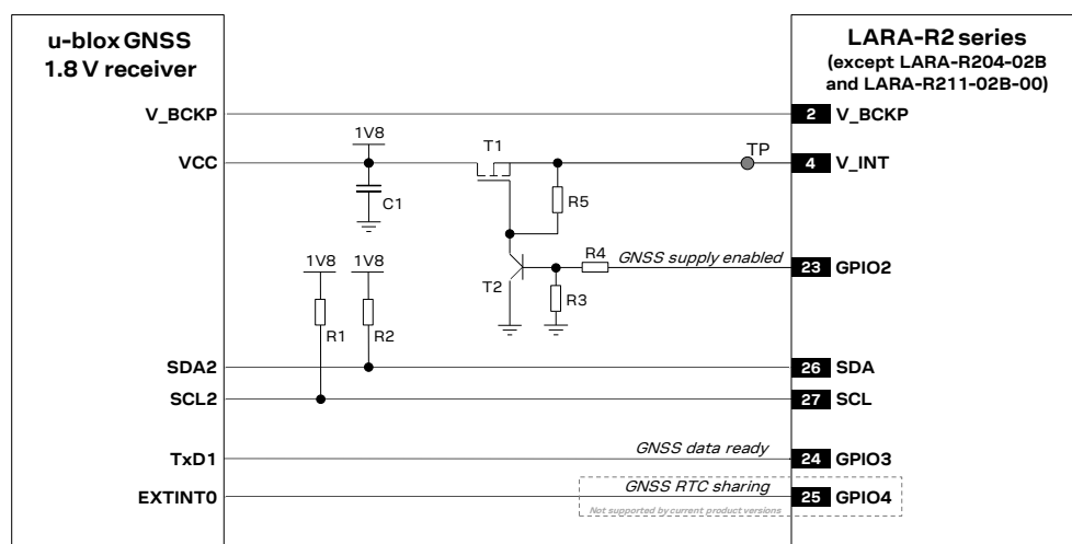
Figure 66: Application circuit for connecting LARA-R2 series modules to u-blox 1.8 V GNSS receivers using V INT as supply
