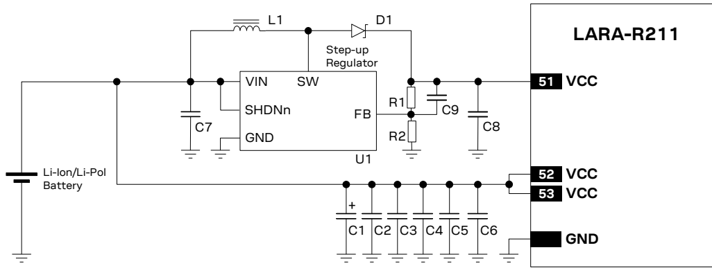
Figure 33: VCC circuit example with a separate supply for LARA-R211 modules
