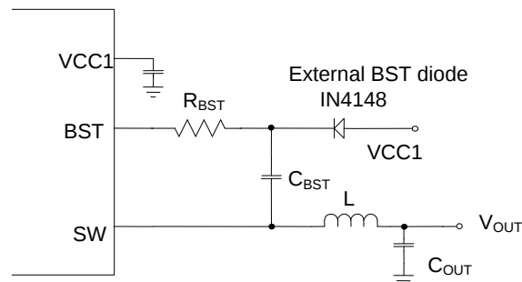
Figure 8: External Bootstrap Diode and Resistor
