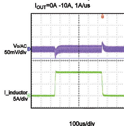
Transient Response
