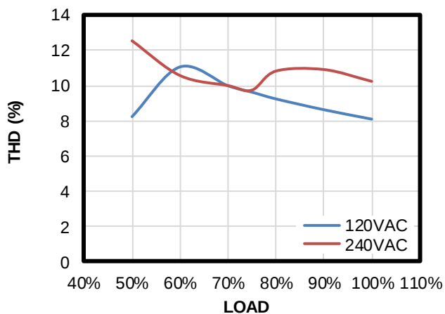
THD
