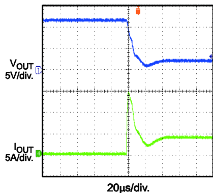
0.6 \Omega Load Connected To Enabled Device
