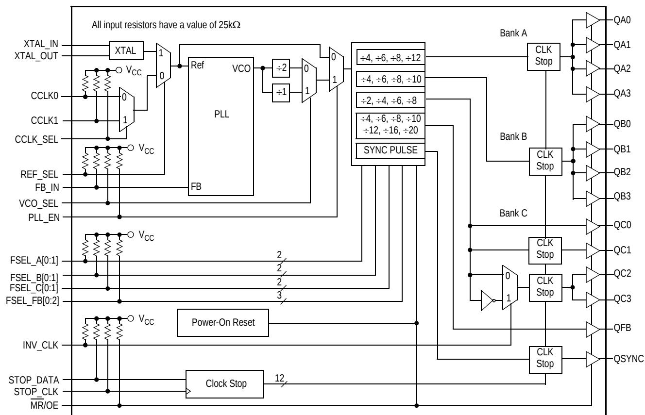
Figure 1. Logic Diagram
