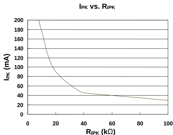
Figure 5: I_{PK} vs. R_{IPK}
