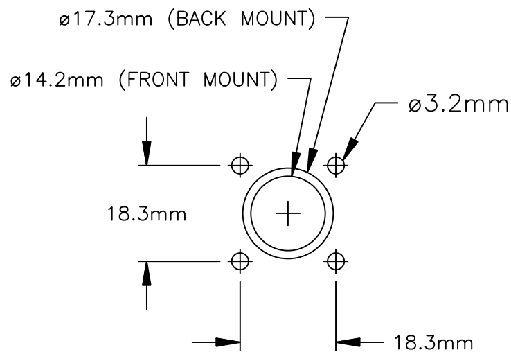
PANEL CUTOUT
